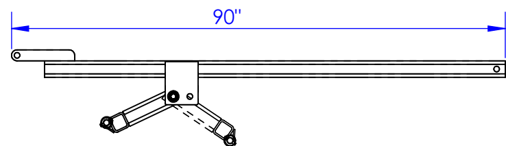
SIDE VIEW SHOWN WITH TRACTOR WHEEL THREE POINT MAST, HYDRA-PHD w/ 12" AUGER DOWN POSITION
