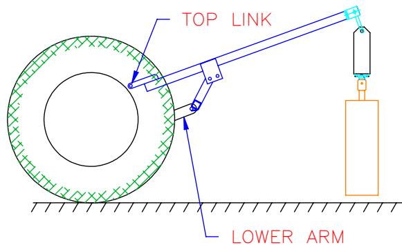
SIDE VIEW SHOWN WITH TRACTOR WHEEL THREE POINT MAST, HYDRA-PHD w/ 12" AUGER UP POSITION
