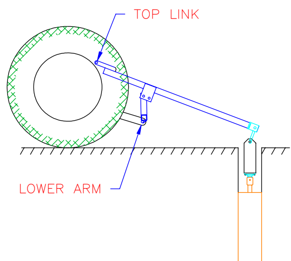
SIDE VIEW SHOWN WITH TRACTOR WHEEL THREE POINT MAST, HYDRA-PHD w/ 12" AUGER DOWN POSITION
